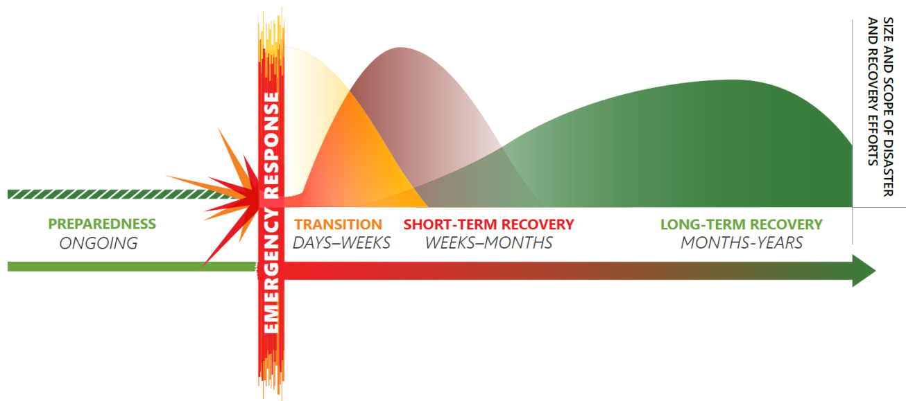
Figure 11: Recovery Continuum
